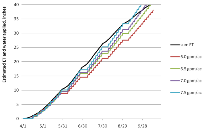
Figure 1. Cumulative estimated ET averaged over 30 years, including cutting effects and irrigation water applied by center pivot at 4 irrigation system capacities for Kimberly, ID conditions. The four horizontal “stair steps” where ET is level result from the harvest periods when it takes a few days for the alfalfa to form new leaves and ET to resume significantly.
