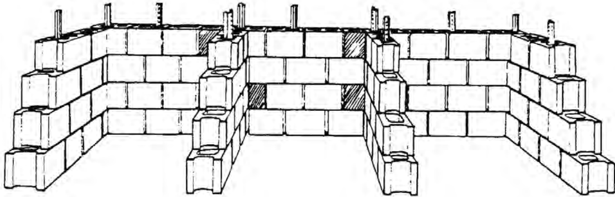
CONCRETE-BLOCK, THREE-BIN TURNING UNIT
